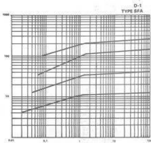
PROSPECTIVE CURRENT IN KA (SYMMETRICAL RMS)
