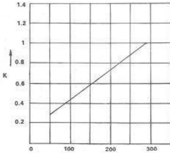
APPLIED VOLTAGE (RMS) FUSE TYPE: SFE
