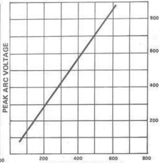
APPLIED VOLTAGE RMS FUSE TYPE: SFD
