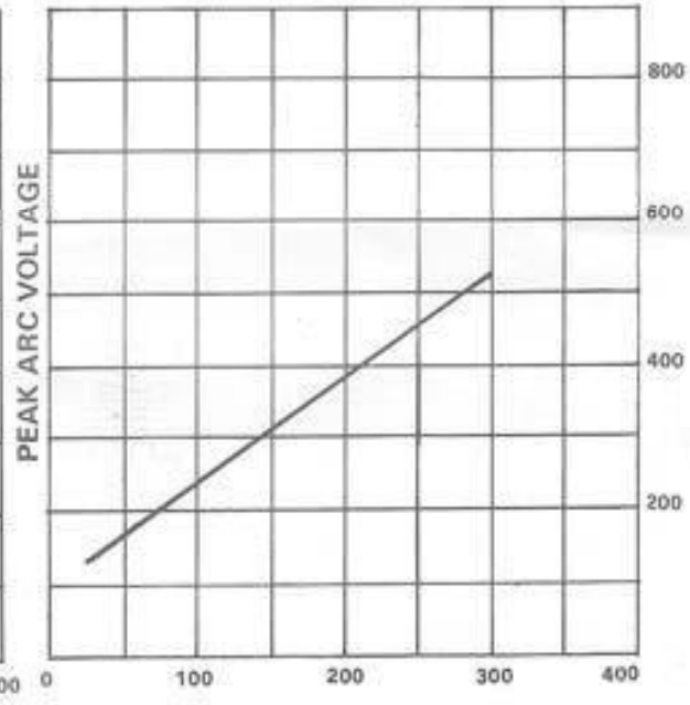
APPLIED VOLTAGE RMS FUSE TYPE: SFC
