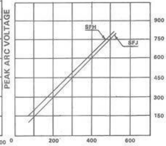
APPLIED VOLTAGE RMS FUSE TYPE: SFH, SFJ
