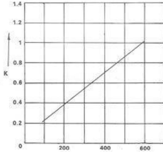
APPLIED VOLTAGE (RMS) FUSE TYPE: SFF
