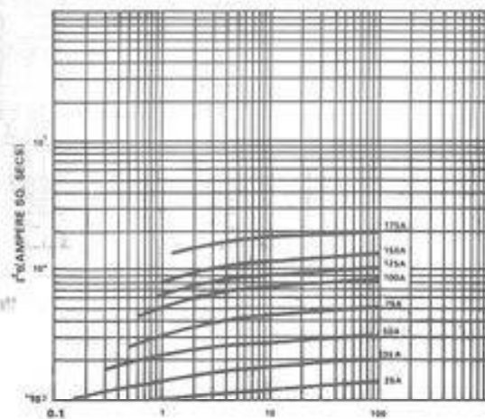
PROSPECTIVE CURRENT IN KA (SYMMETRICAL RMS)
