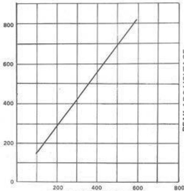
APPLIED VOLTAGE R.M.S. FUSE TYPE: SFB
