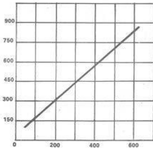
APPLIED VOLTAGE RMS FUSE TYPE: SFF
